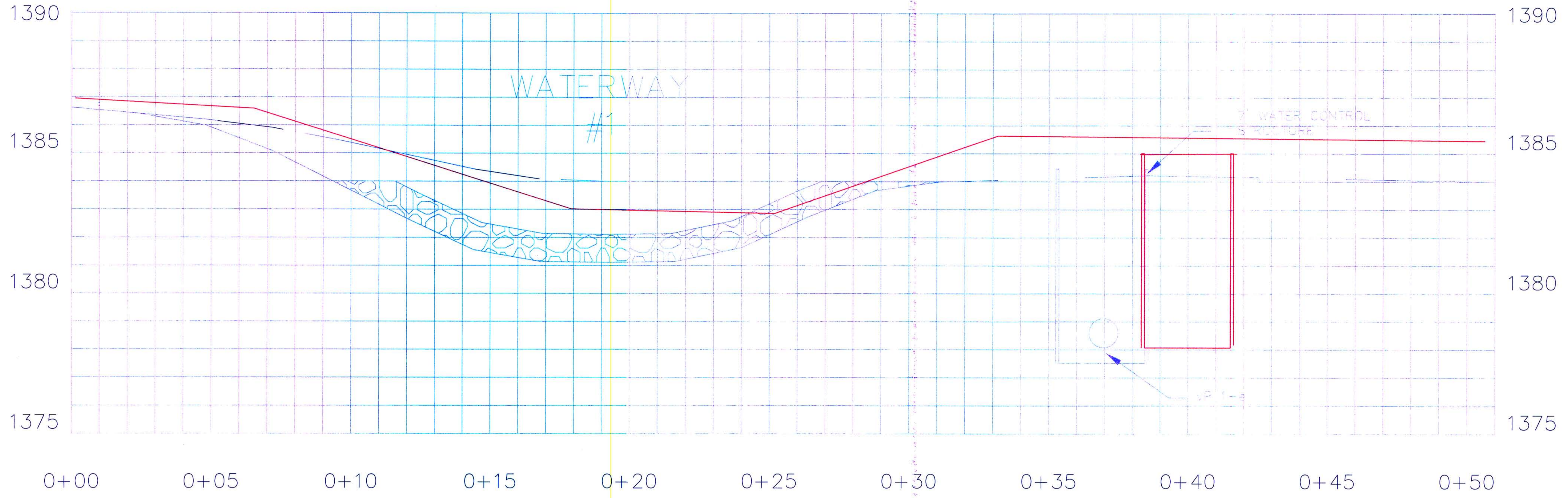
SECTION E-E
